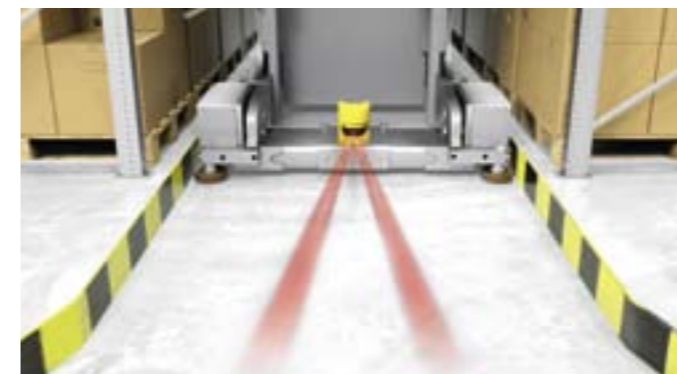
Mobile personal protective equipment with laser scanner
